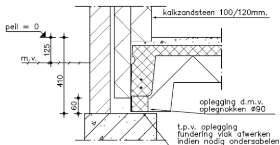
kalkzandsteendetail 6
