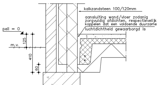
kalkzandsteendetail 5
