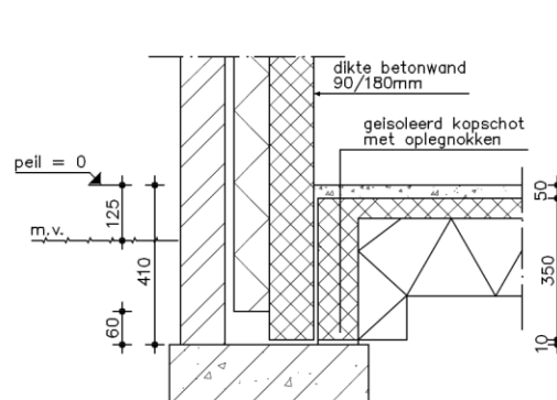
beton/giet detail 1B/G
